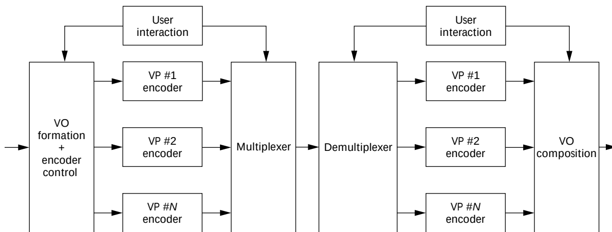
Figure 3. General structure of the MPEG-4 video encoder/decoder. (Note, VO represents video object.)
