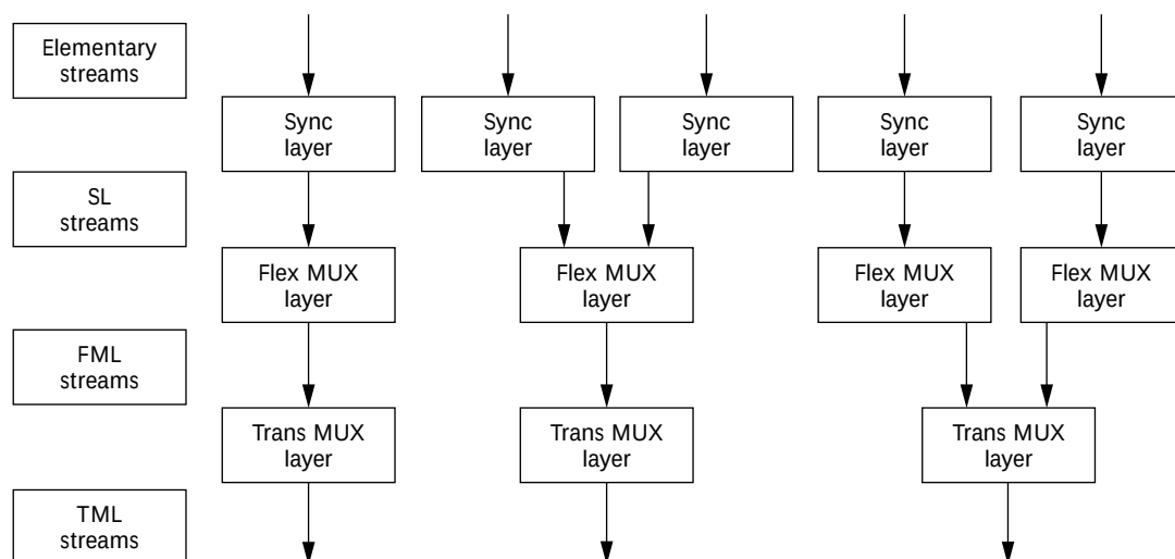
Figure 2. General structure of the MPEG-4 multiplex. Different cases have multiple SL streams multiplexed in one FML stream and multiple FML streams multiplexed in one TML stream.
