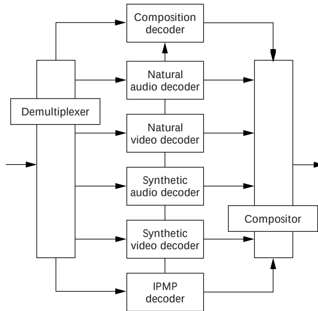
Figure 1. MPEG-4 high-level system architecture (receiver terminal).
